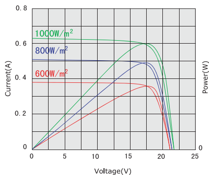
Electrical Performance cell temperature: 25 °C
